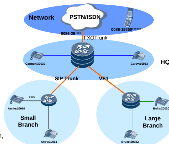
Figure 1: Huawei Enterprise Routers Voice Network Topology
