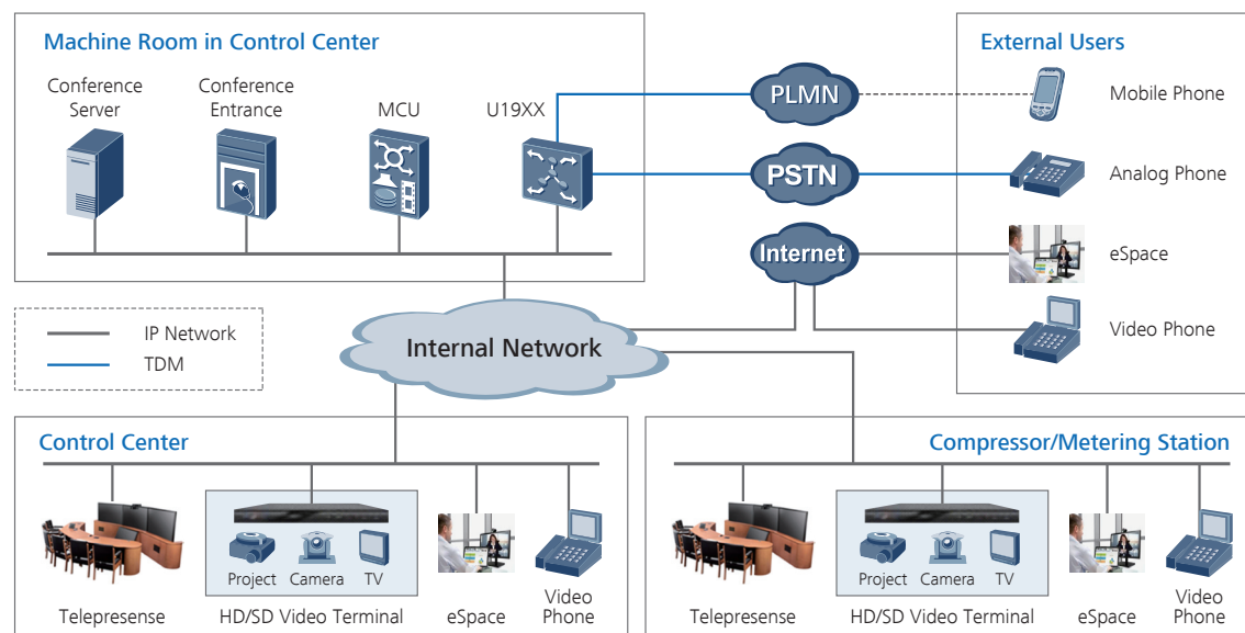
Figure 3 Multiterminal convergence conference system
