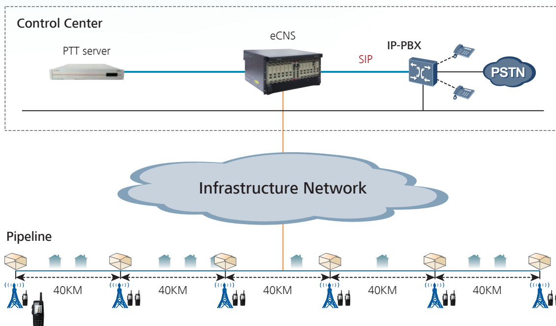
Figure 4 All-in-one voice service system
