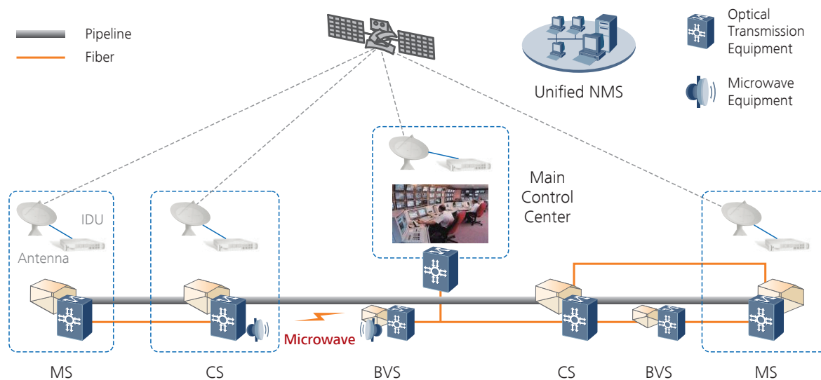
Figure 2 Digital pipeline backbone network solution
