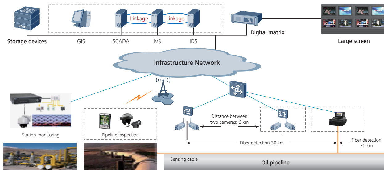
Figure 5 Digital pipeline integrated security solution
