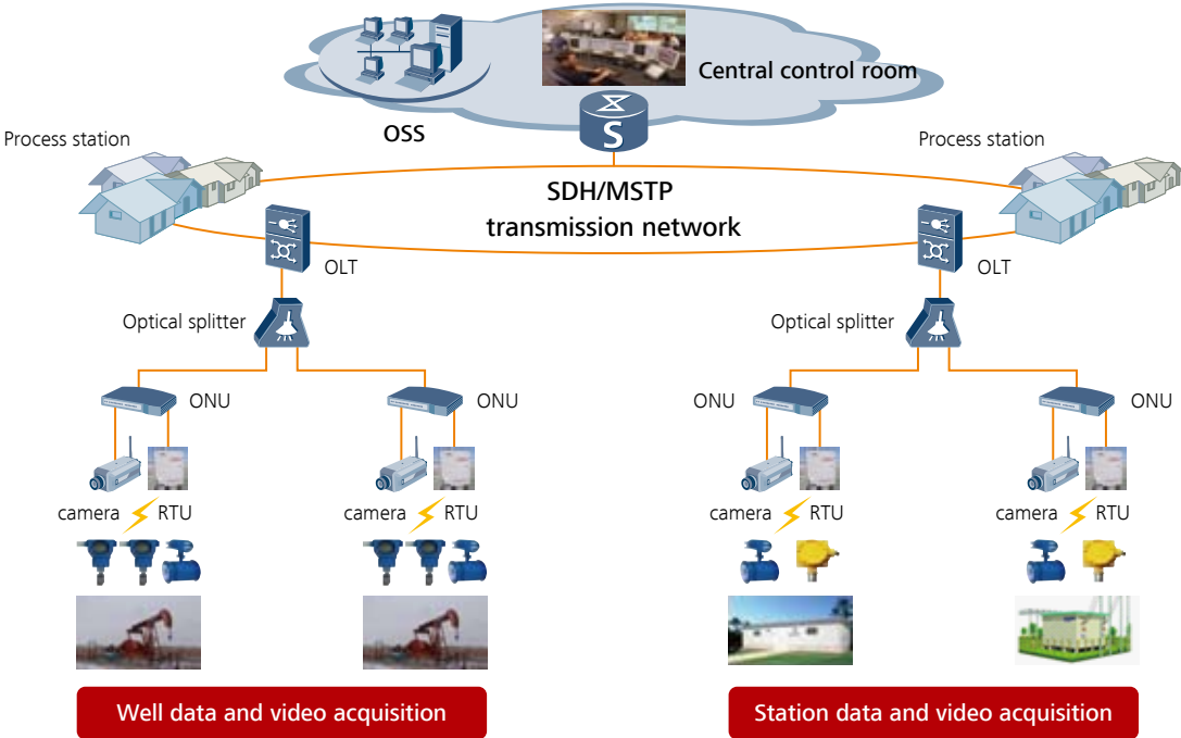
Figure 4 Oil and gas xPON network solution
