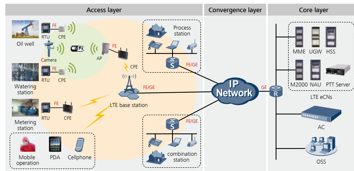
Figure 2 LTE+WLAN network for oil and gas production
