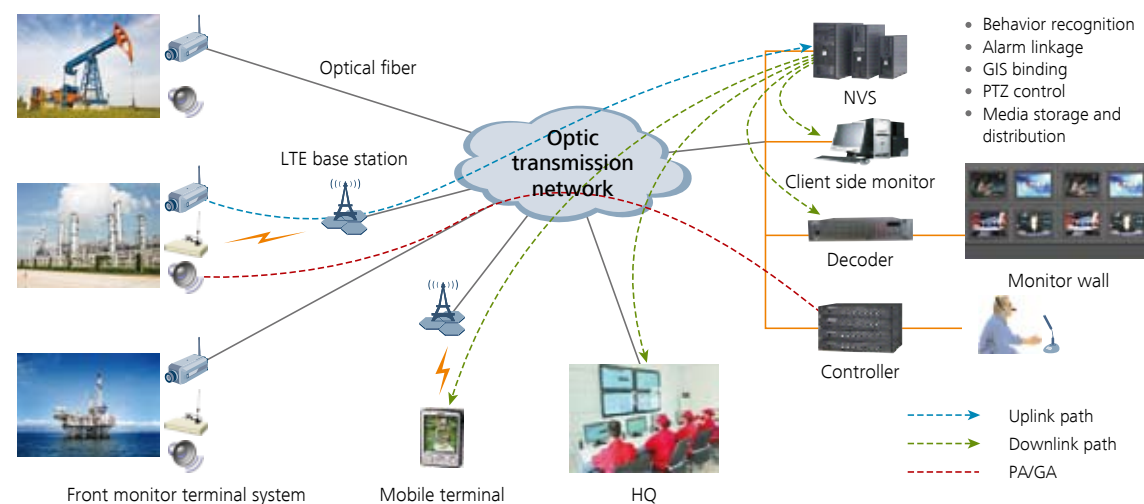
Figure 6 Digital production video surveillance solution
