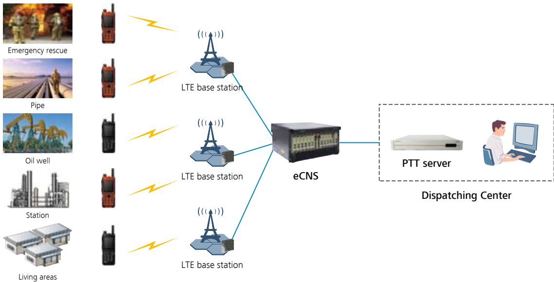
Figure 5 Multimedia digital trunking communication solution
