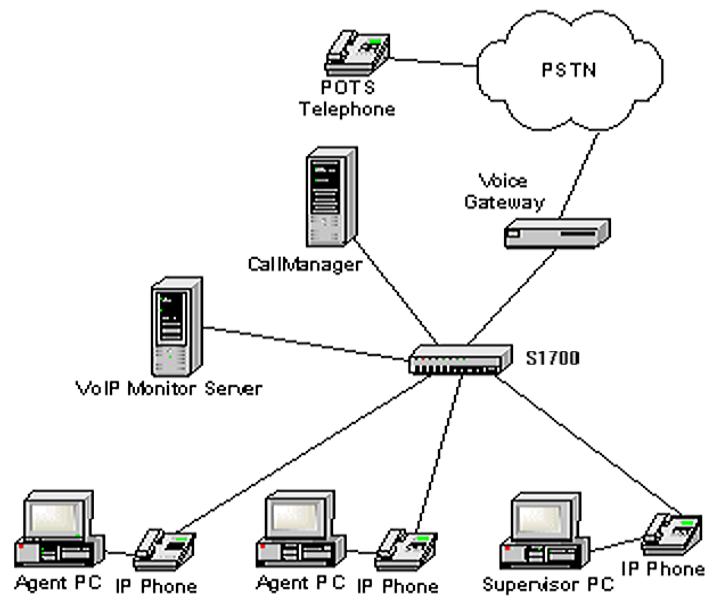
Figure 5-2 Voice VLAN
