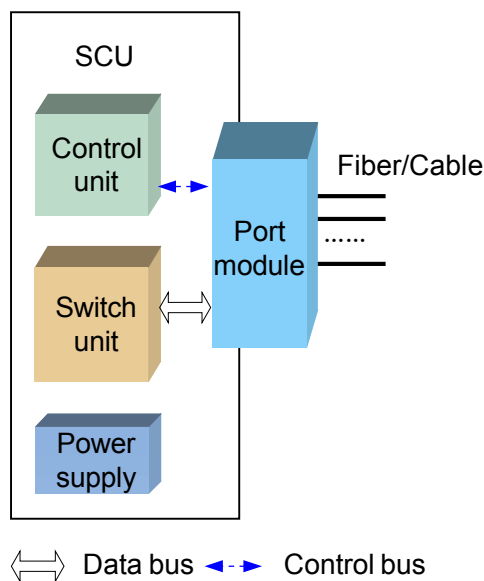
Figure 2-1 Logical structure of hardware modules of the S3700
