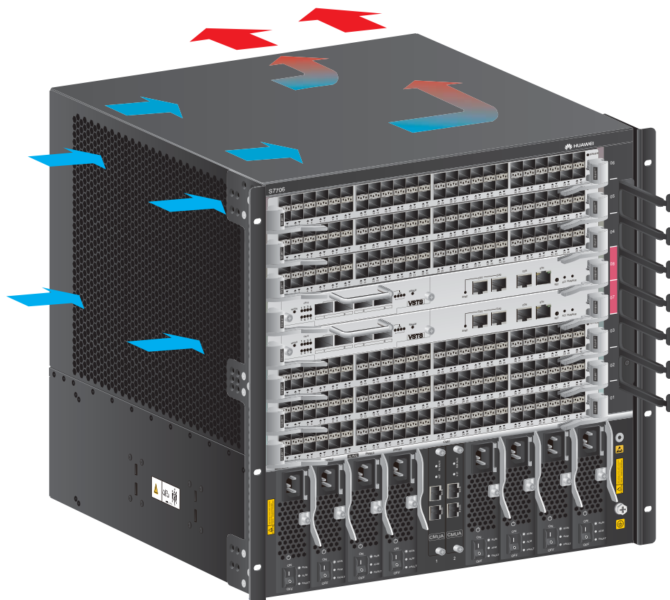
Figure 3-24 Airflow in the S7706 chassis
