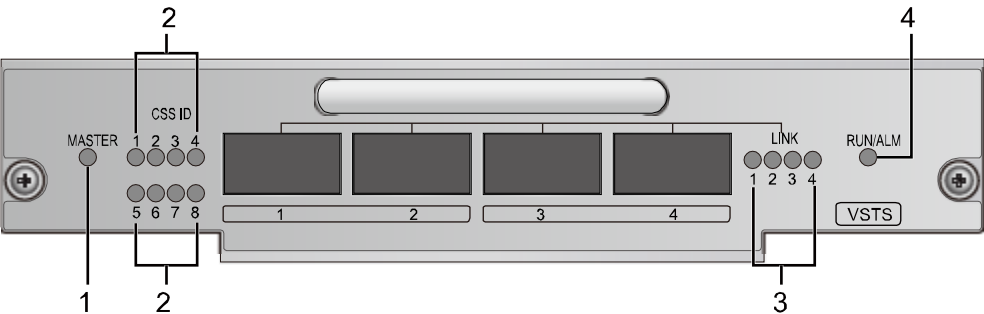
Figure 6-17 Indicators on the ES02VSTSA
