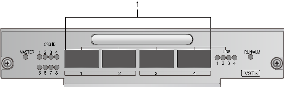
Figure 6-18 Ports on the ES02VSTSA
