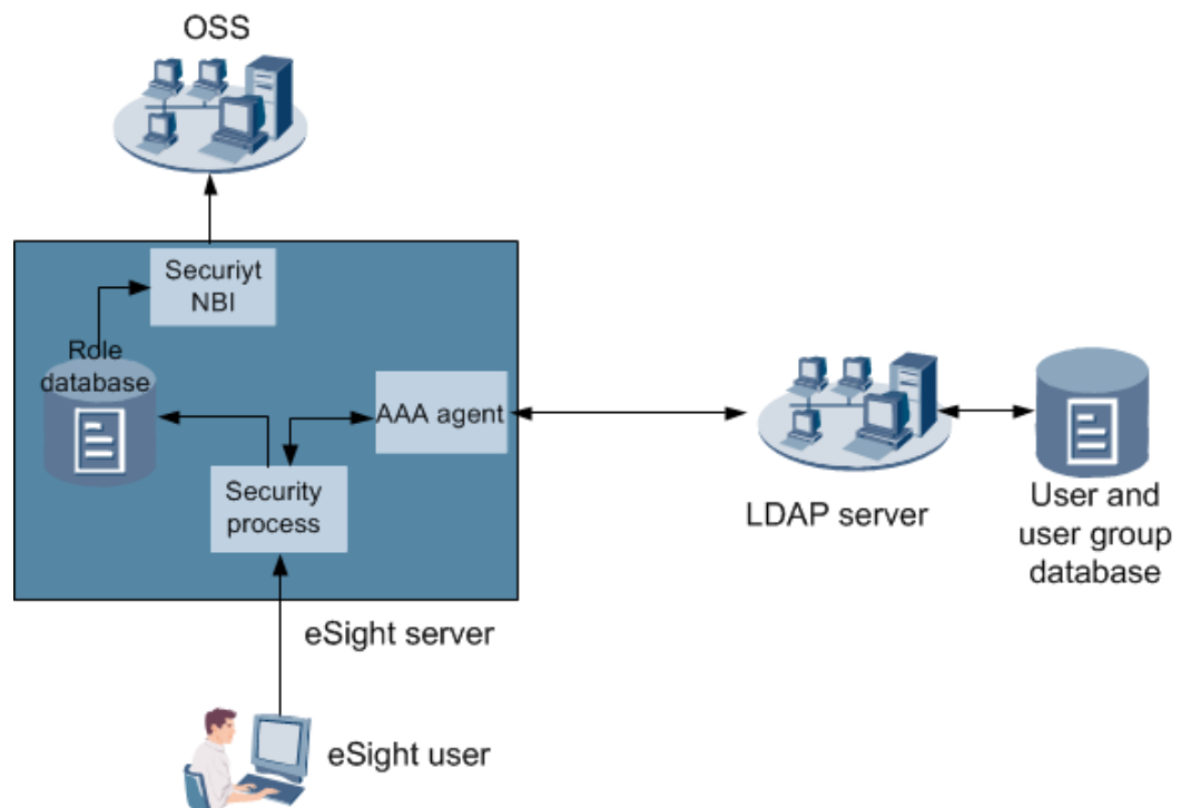
Figure 4-3 LDAP authentication
