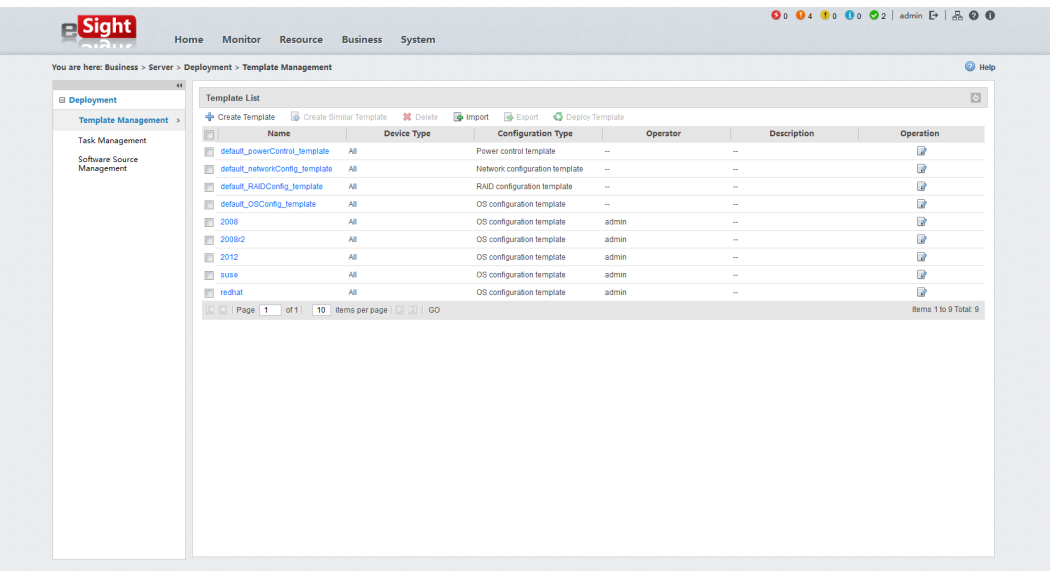
Figure 4-182 Configuration template
