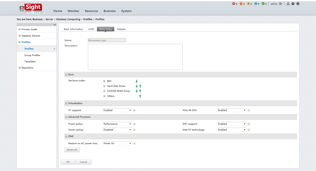
Figure 4-179 Profile sample
