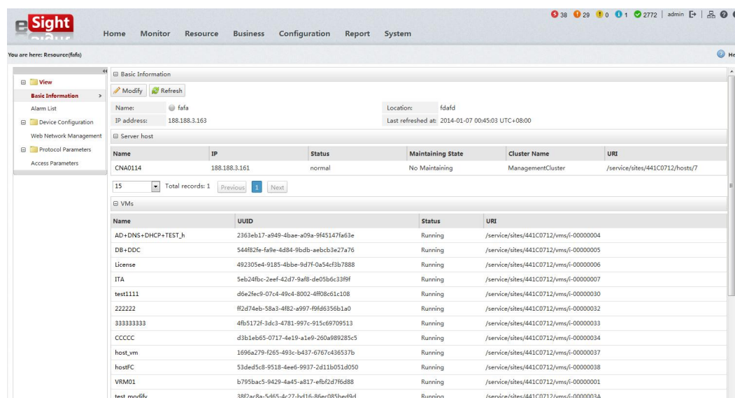
Figure 4-63 NE manager
