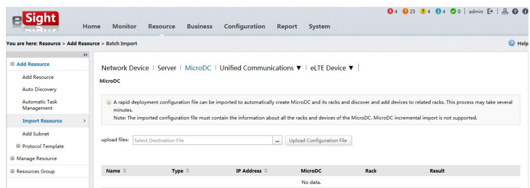
Figure 4-71 Batch import
