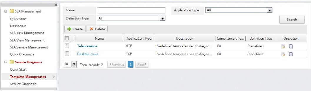
Figure 4-123 Template management
