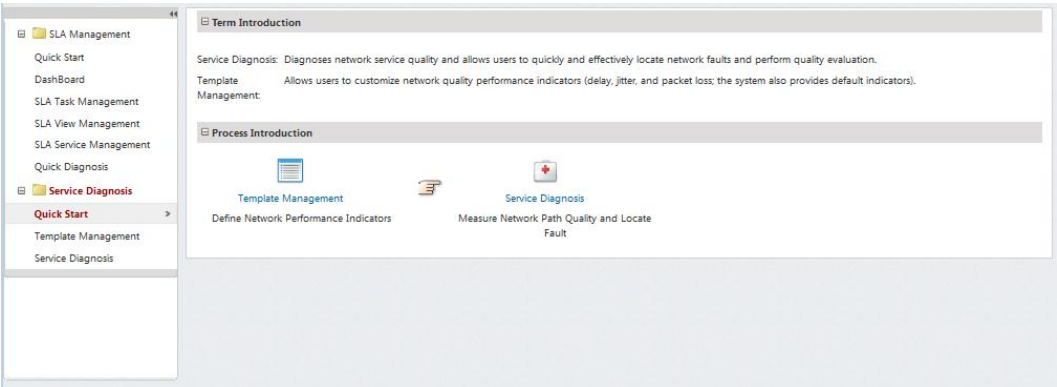
Figure 4-122 Quick Start
