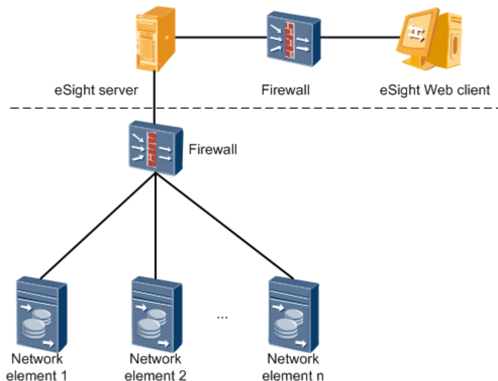
Figure 3-1 Standalone mode
