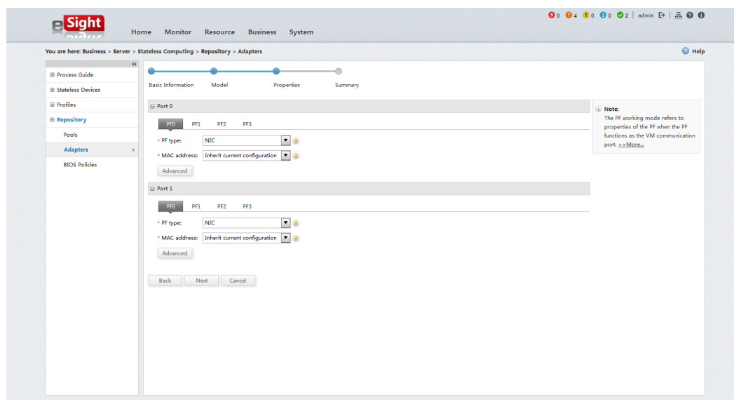
Figure 4-177 Adapter configuration
