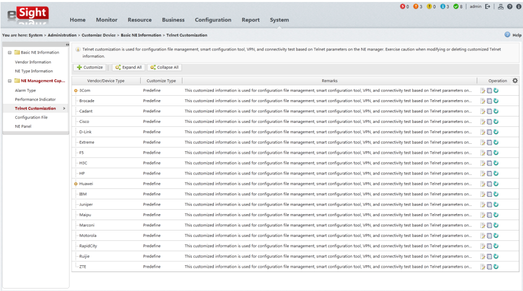
Figure 4-57 Telnet customization
