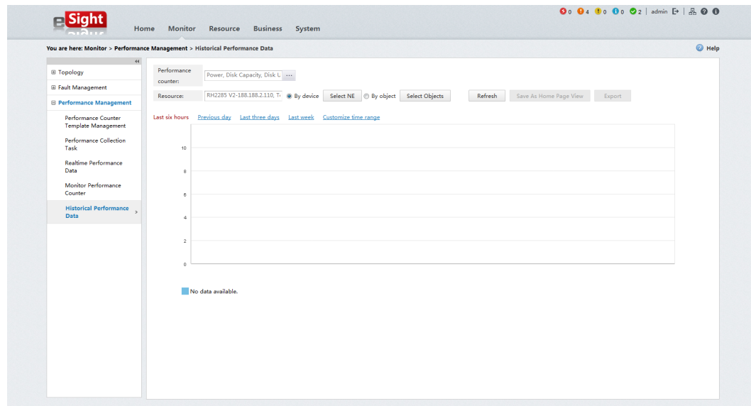
Figure 4-62 Performance analysis
