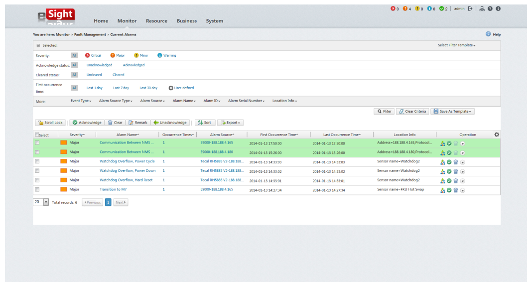
Figure 4-61 Alarm monitoring
