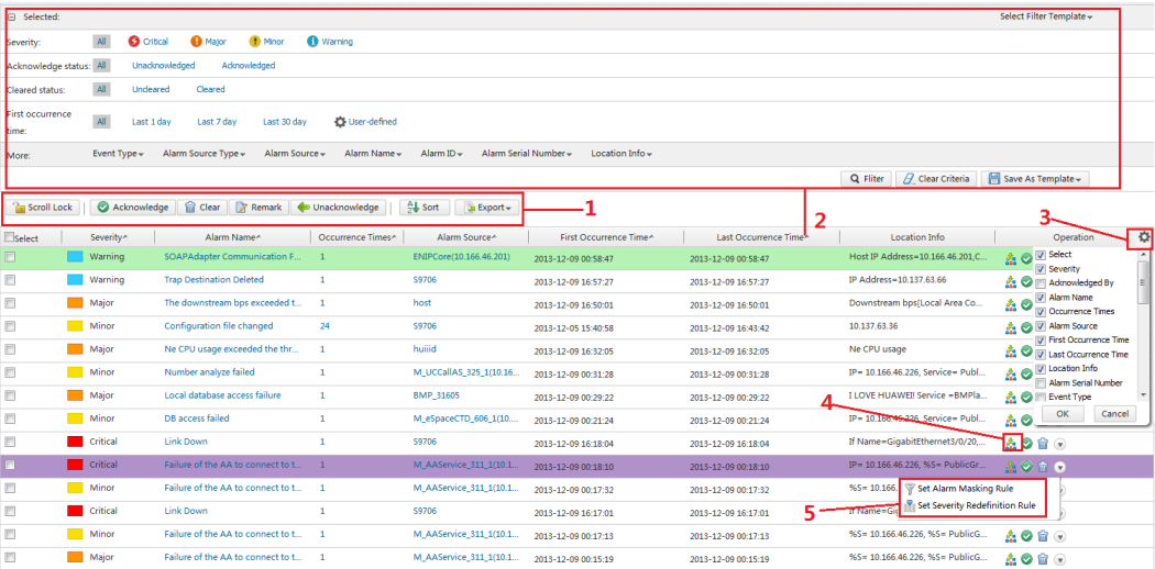
Figure 4-7 Current Alarms
