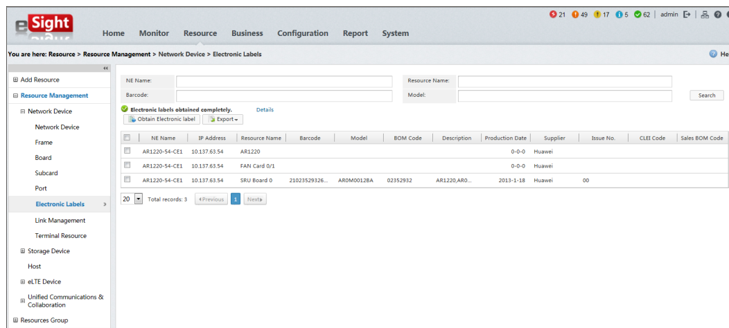
Figure 4-20 Electronic Labels
