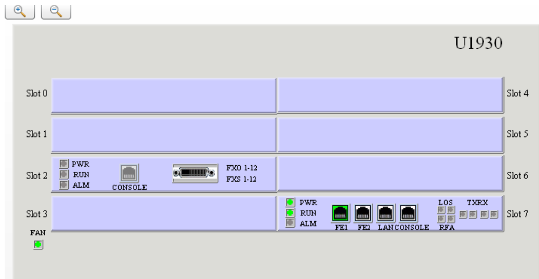
Figure 4-74 Device panel
