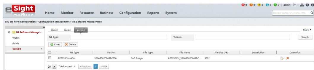
Figure 4-47 Version Management
