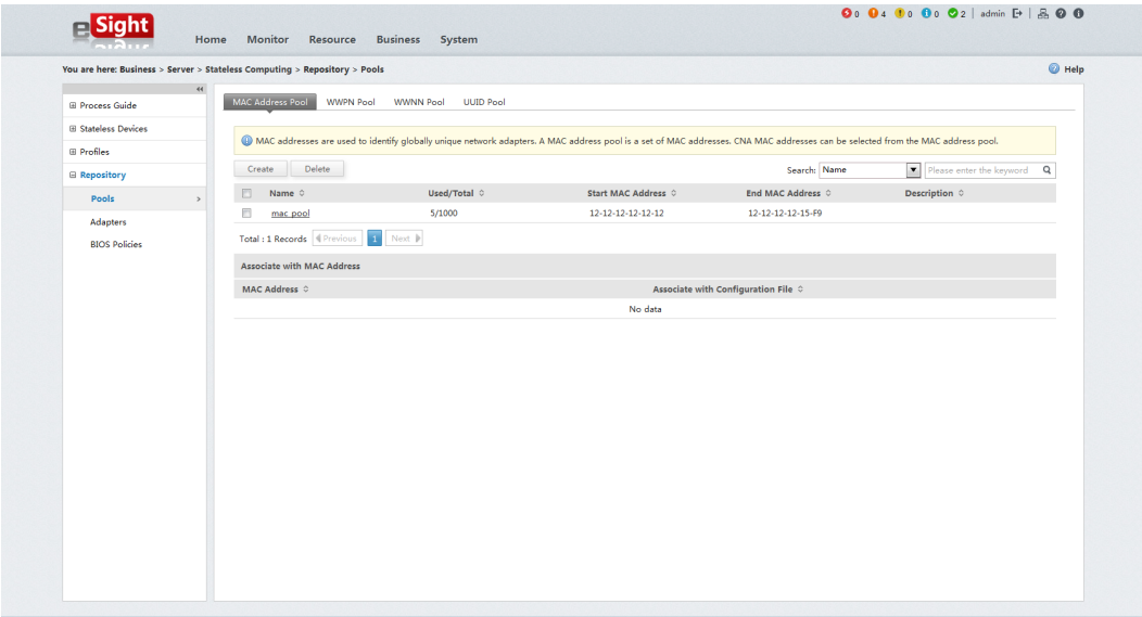
Figure 4-176 Pool configuration
