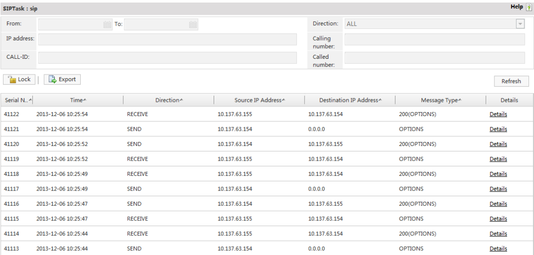
Figure 4-58 Signaling tracing
