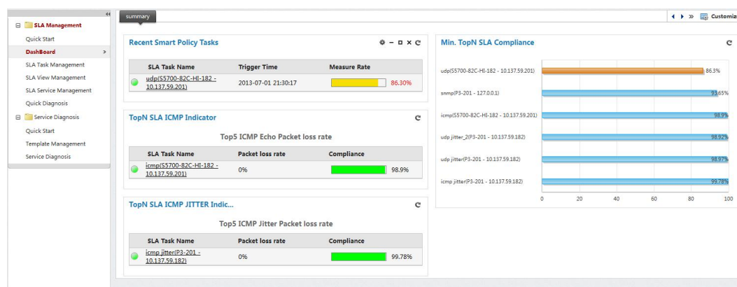
Figure 4-114 SLA Dashboard
