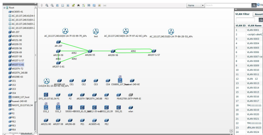
Figure 4-35 VLAN topology
